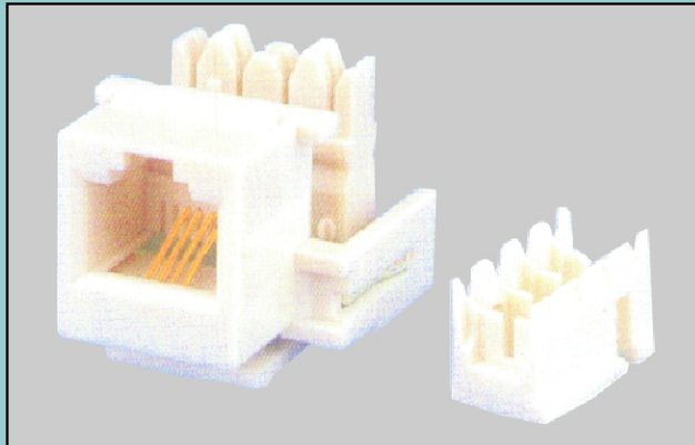
1496 - TELEPHONE JACK RJ 11, 6P4C, 2 line, Punch Type
